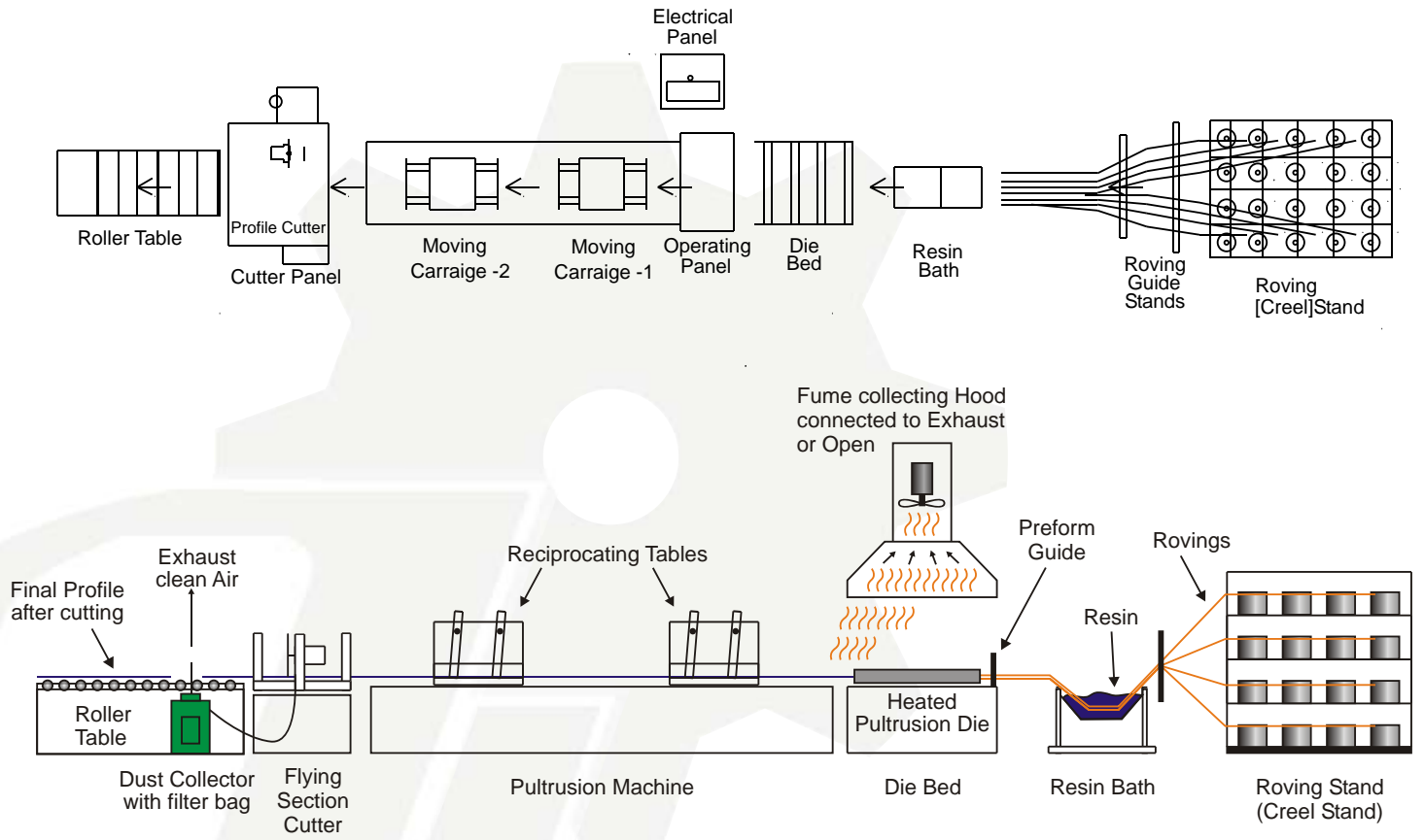
Typical Pultrusion Machine Layout
